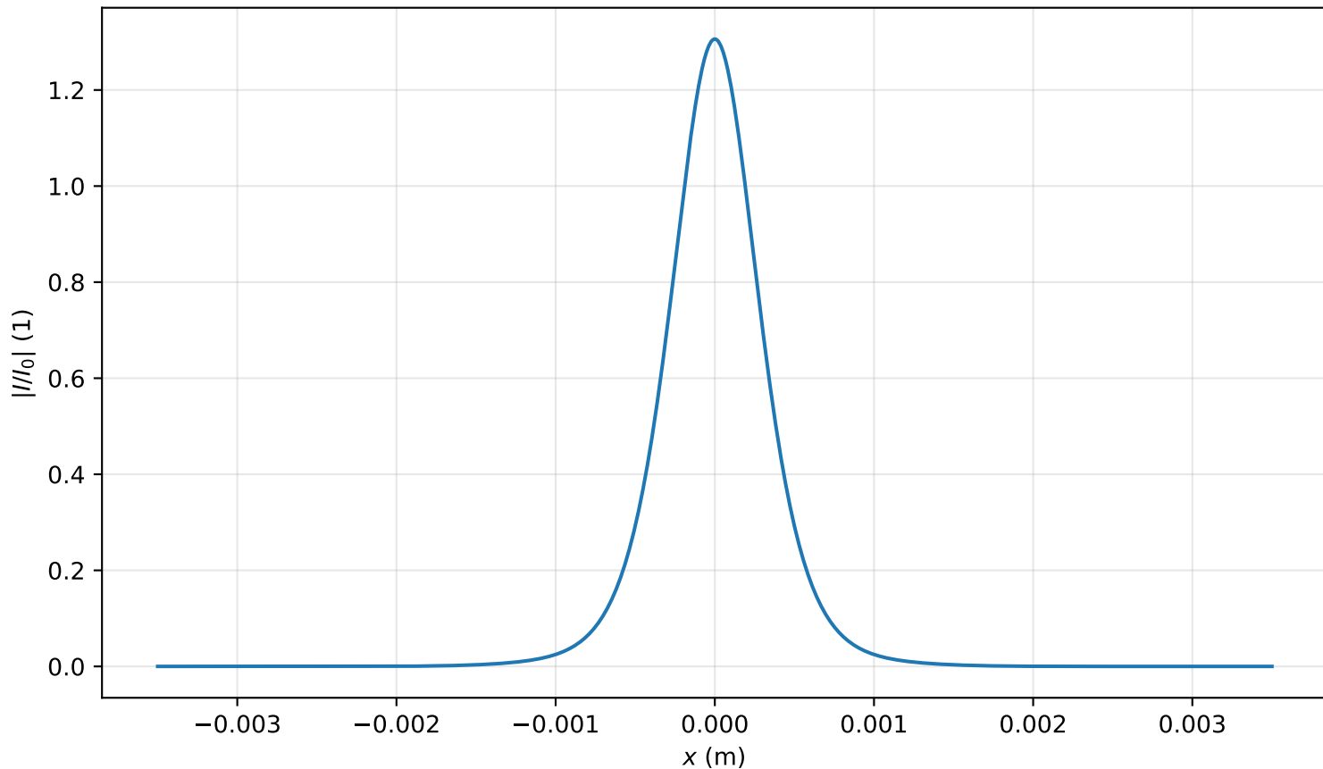
Intensity profile I(x, y = 0, z = 2.070m)/I_0 , P_{in}=0.8P_{cr} , artificial time
